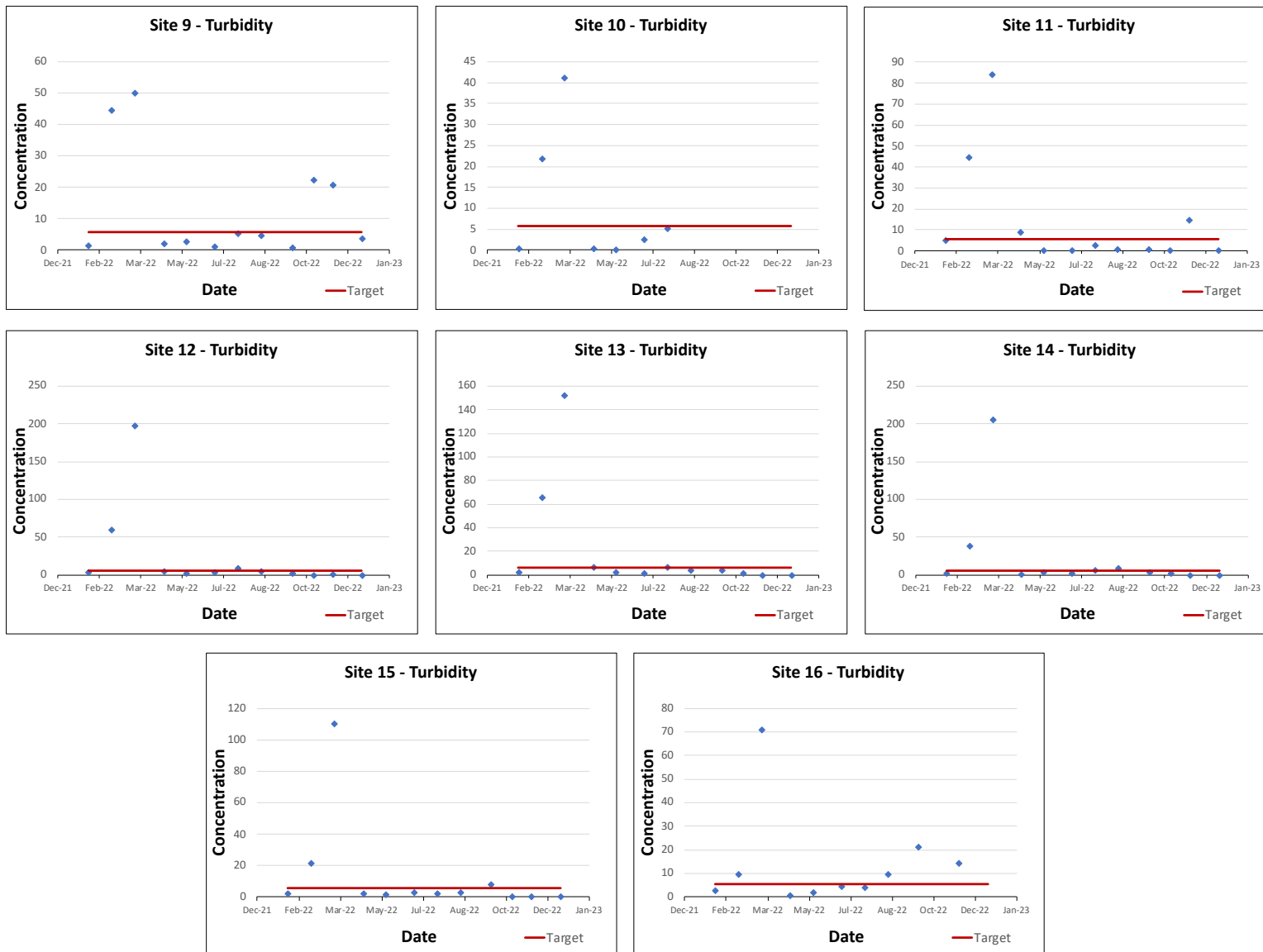
Figure 30. Turbidity measurements in Upper Sugar Creek Watershed samples sites from January 2022-December 2022.
