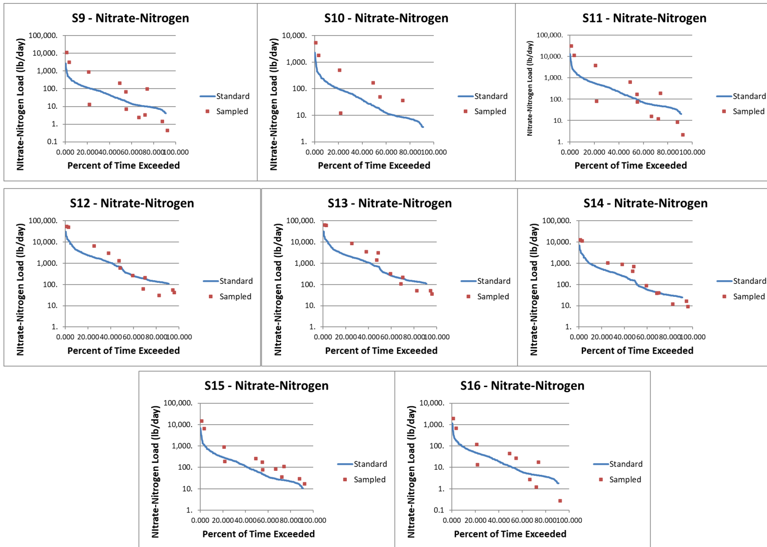
Figure 35. Nitrate-nitrogen load duration curves for Upper Sugar Creek Watershed samples sites from January 2022-December 2022.
