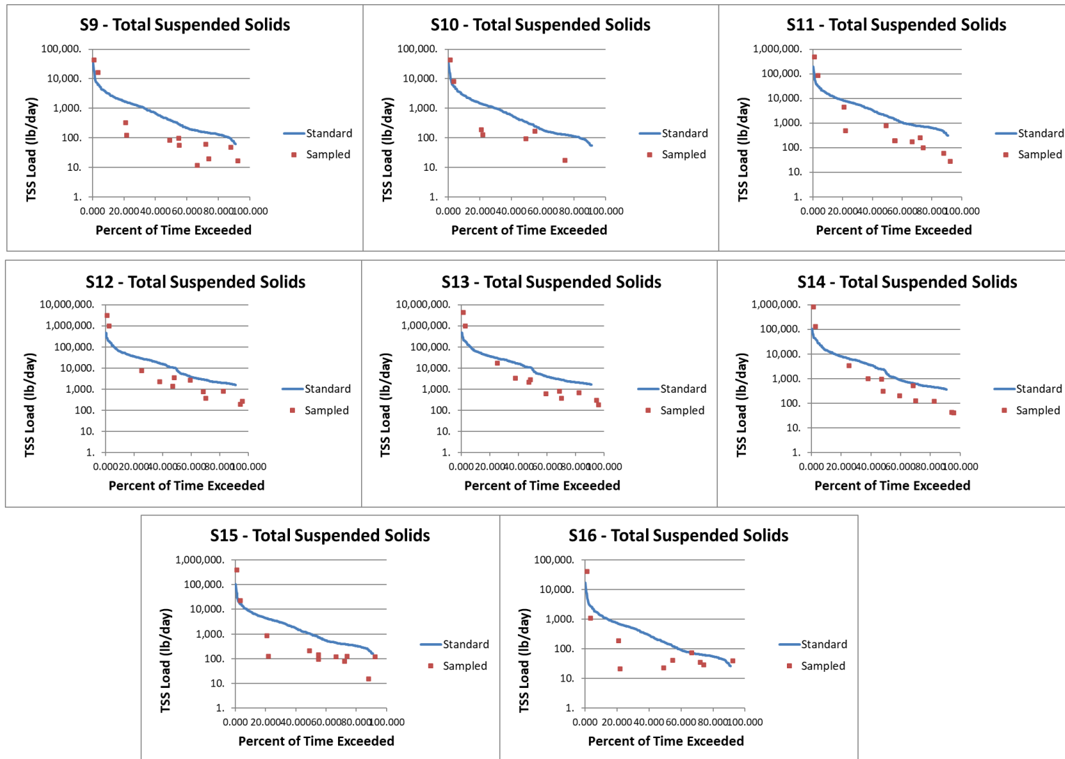
Figure 37. Total suspended solids load curves for Upper Sugar Creek Watershed samples sites from January 2022-December 2022.
