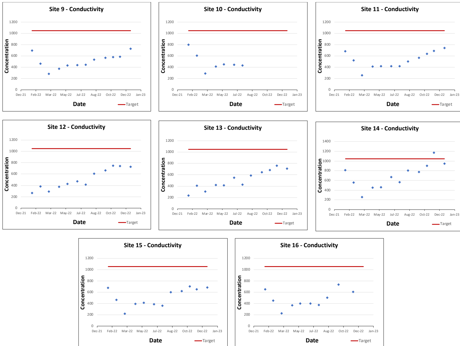
Figure 29. Conductivity measurements in Upper Sugar Creek Watershed samples sites from January 2022-December 2022.
