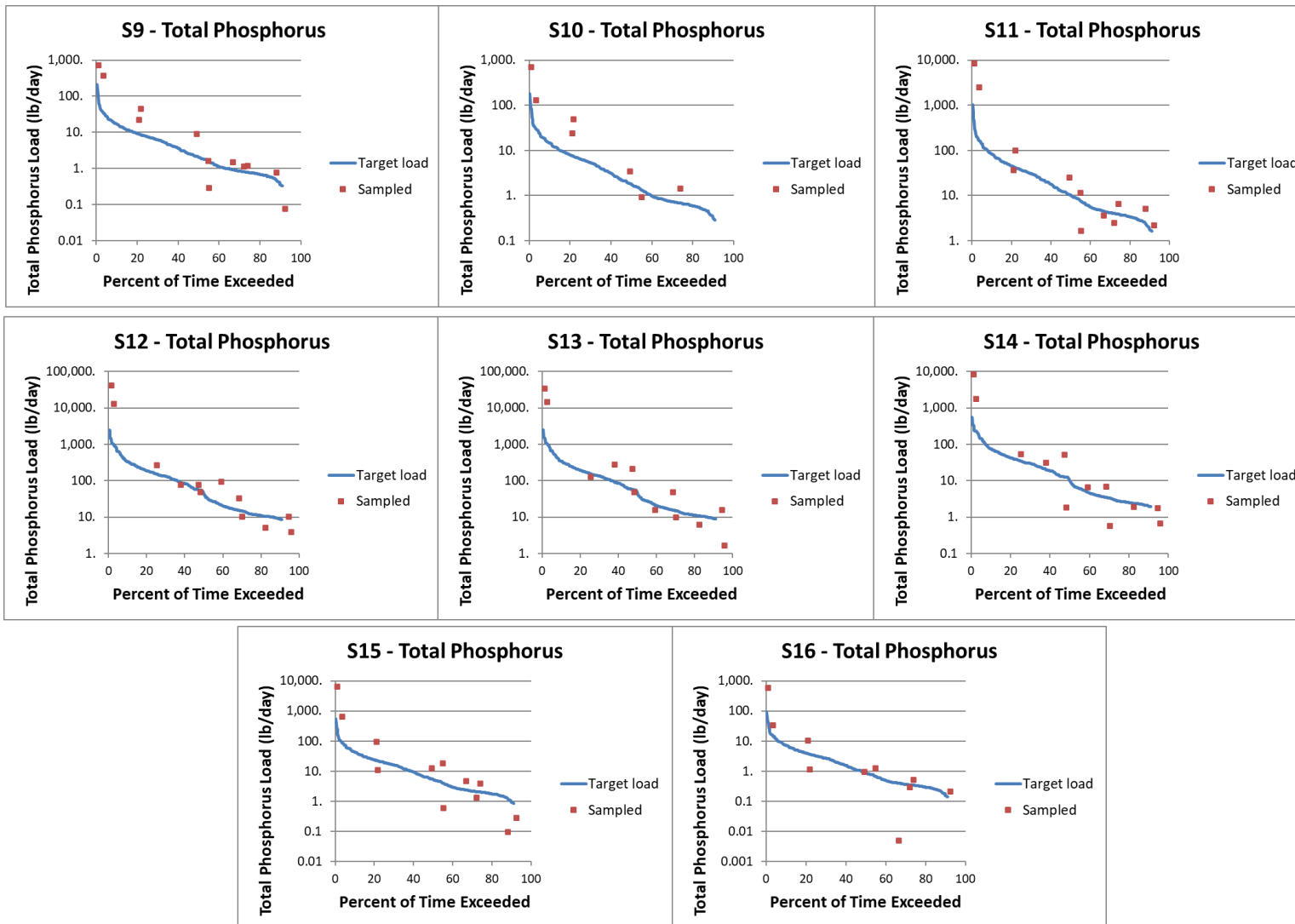
Figure 40. Total phosphorus load duration curves for Upper Sugar Creek Watershed samples sites from January 2022-December 2022.
