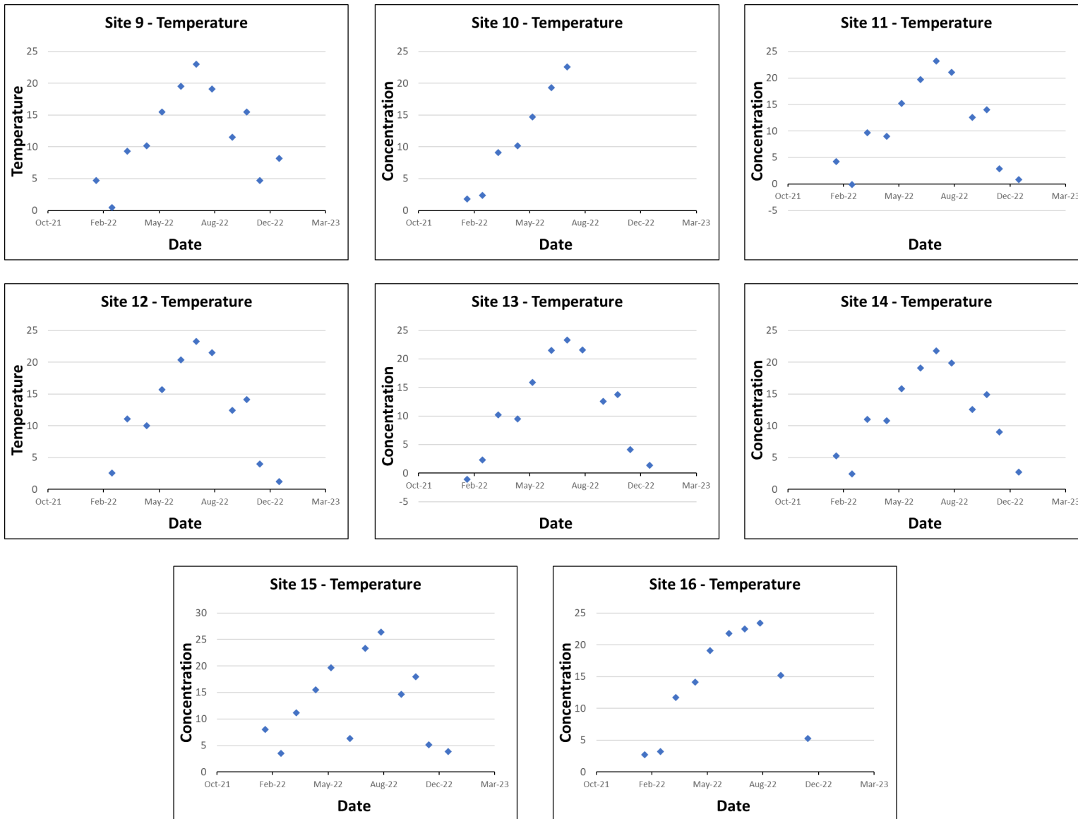
Figure 30. Temperature measurements in Upper Sugar Creek Watershed samples sites from January 2022-December 2022. Note differences in scale along the concentration (y) axis.
